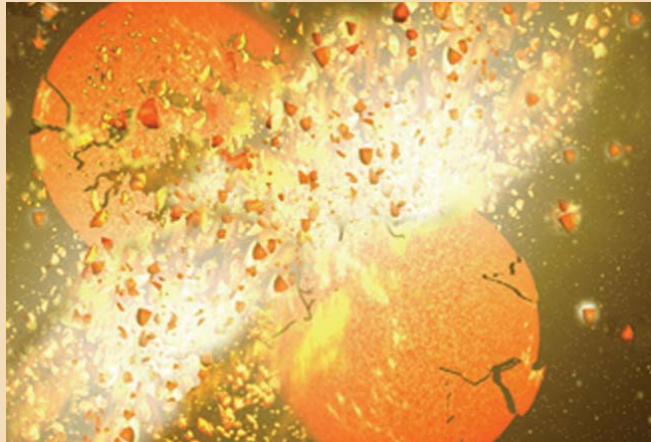
An artist's rendering of a possible collision scenario between two huge asteroids or tiny planets. UF astronomers say such a collision may be the cause of the lopsided appearance of Beta Pictoris.
